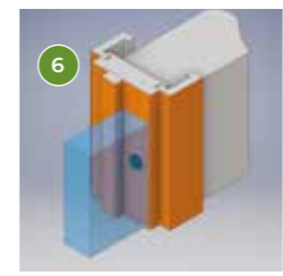
6 Quick2Fit Pads are fitted to the edge of the door to help maintain the essential 3-4mm gap required for fire certification.
